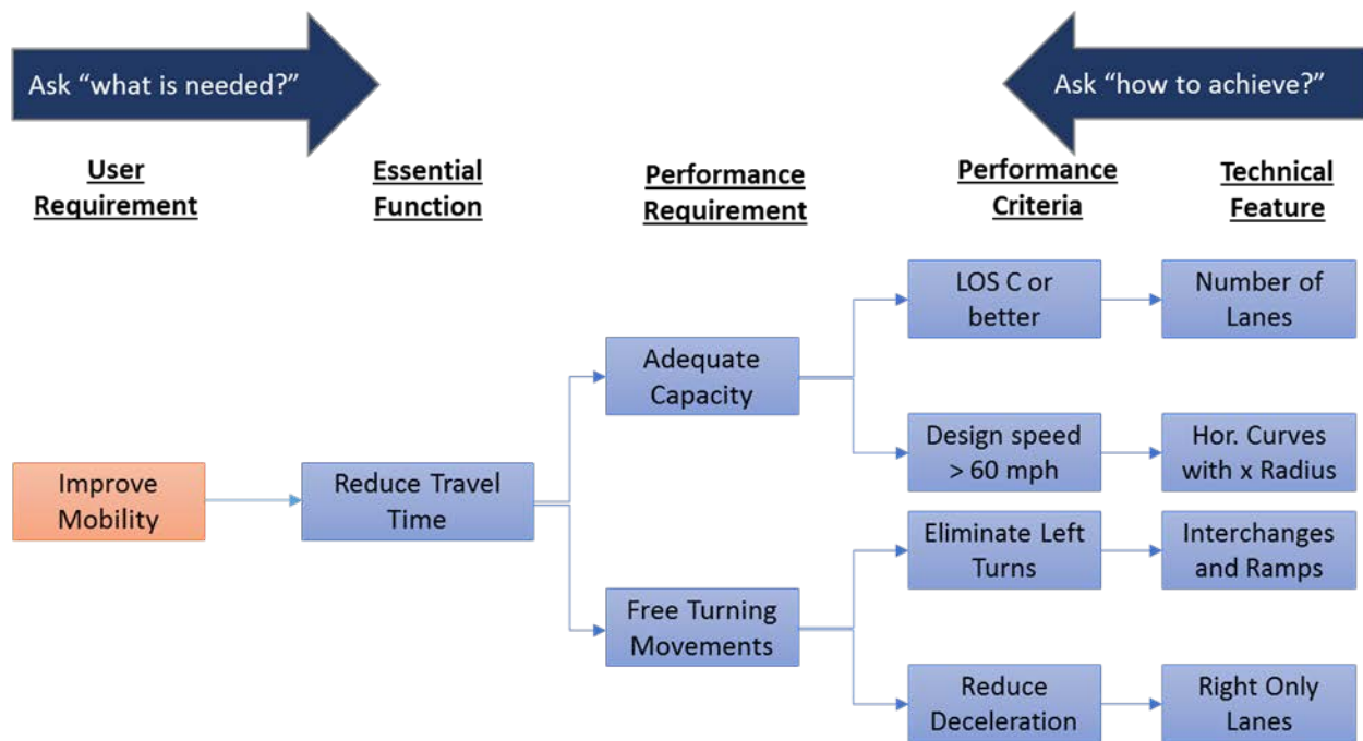
Figure 5. Sample Analysis of Performance Elements using Function Analysis System Technique
